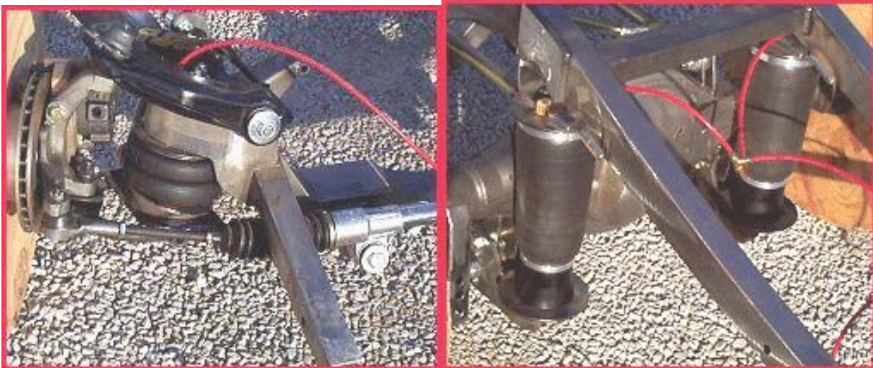
Mustang II front end fully compressed
