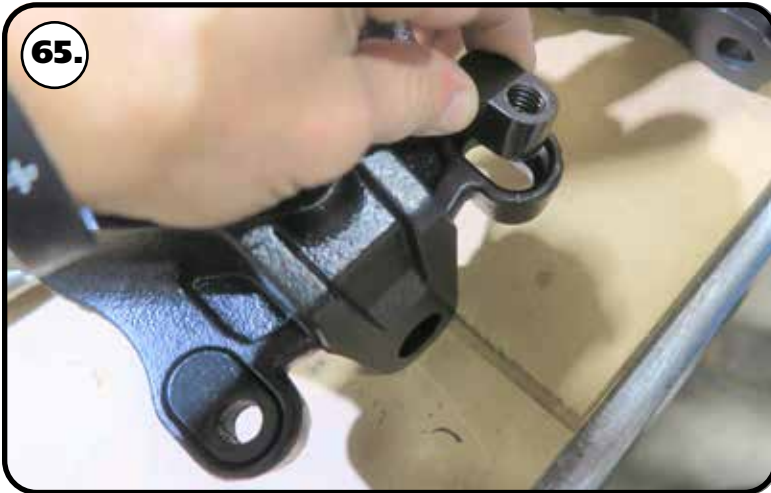
65. Insert the steering arm slugs into the spindle with the threads to the bottom of the spindle,
